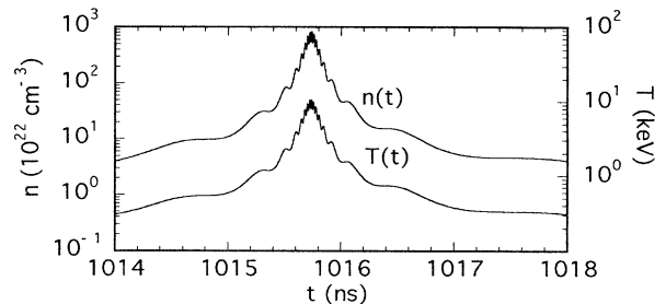
FIG. 5. Plots of the density and temperature of the fiber plasma as a function of time.
