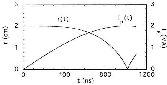
FIG. 2. Outer pinch current and outer pinch radius as a function of time.
