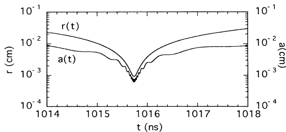
FIG. 3. Plots of the outer pinch radius and the inner fiber radius as a function of time during the last phase of compression.
