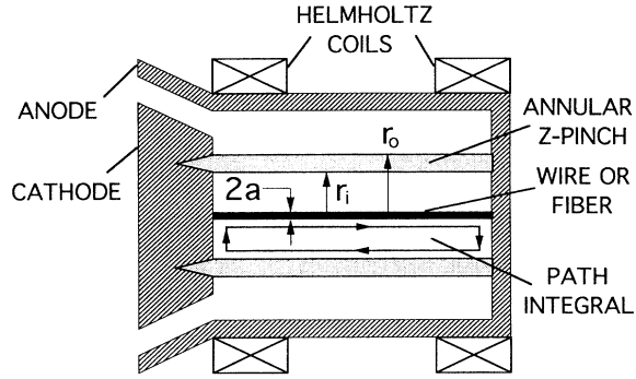
FIG. 1. Schematic illustration of the staged Z-pinch configuration.
