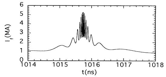
FIG. 4. Plot of the current through the fiber as a function of time.
